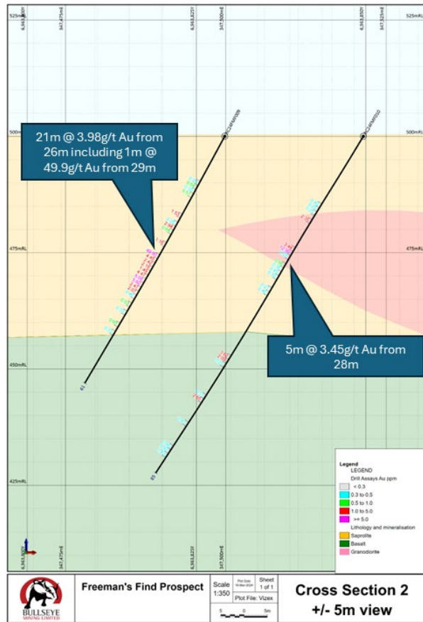
Figure 8 | Section 2 Cross section from the Freeman's Find Prospect. All highlighted significant intersections refer to ASX announcement dated 18 March 2024
