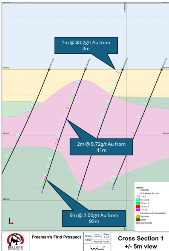
Figure 7 | Section 1 Cross section from the northern edge of the Freeman's Find Prospect. All highlighted significant intersections refer to ASX announcement dated 18 March 2024
